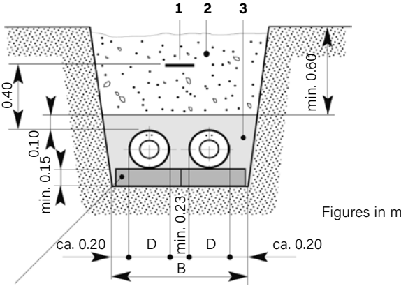
Trench profile, 2 COOLMANT pipes (Ø 125 - Ø 315)
