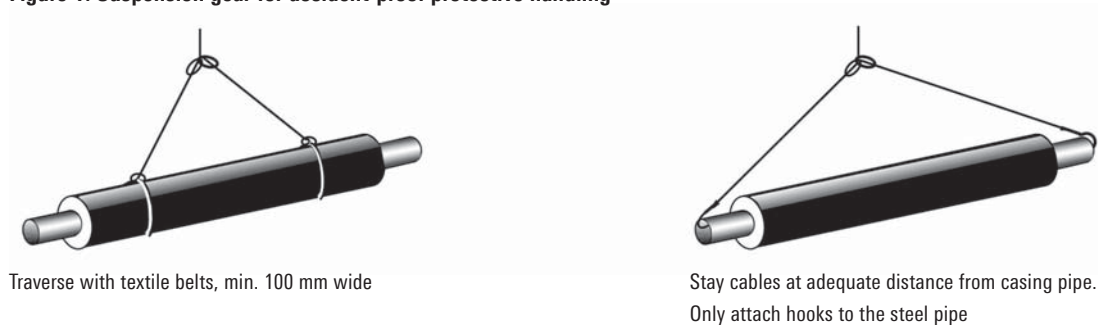
Figure 1: Suspension gear for accident-proof protective handling
