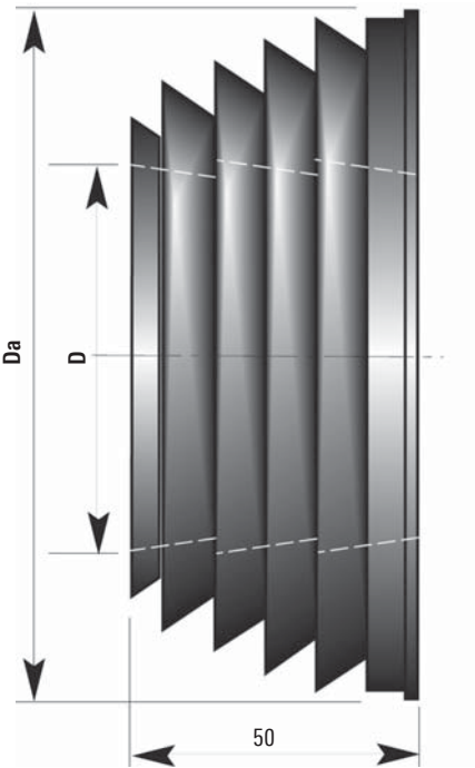
Wall sealing ring
